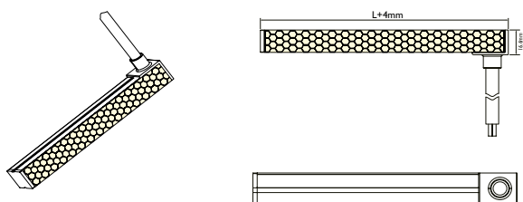
IP67 No dark cap - Side outlet
