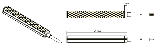
IP67 No dark cap - Axis outlet
