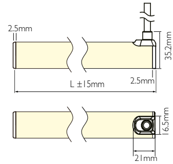
IP67 molded end cap - Side Outlet
