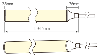
IP67 molded end cap - Axis Outlet
