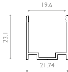
A4333 Moldable groove White (cannot be upside down) 1000mm
