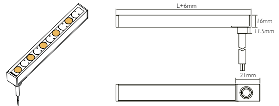
IP67 No dark Endcap - Bottom outlet
