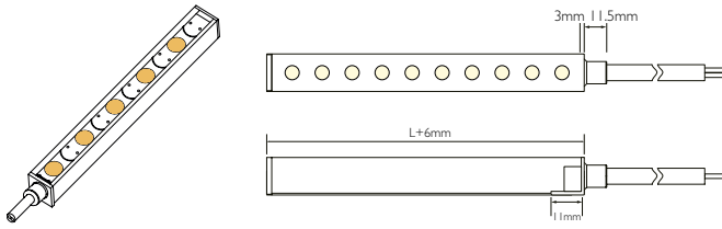
IP67 No dark Endcap - Axis outlet
