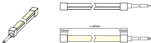
IP67 Glued Endcap - Axis outlet
