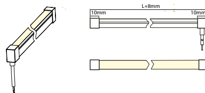
IP67 Glued Endcap - Bottom outlet
