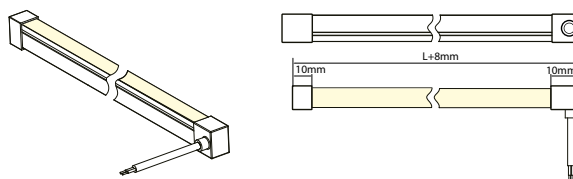
IP67 Glued Endcap - Left side outlet
