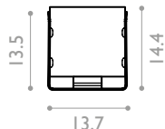
A4401 Moldable Groove 500mm (cannot be used upside down)
