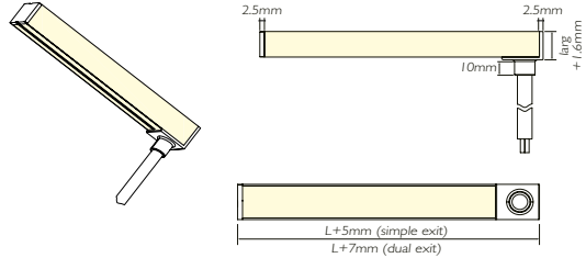
IP67 No Dark Endcap - Left side outlet
