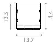
A440I Moldable Groove 500mm (cannot be used upside down)
