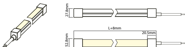
IP67 Glued cap - Axis outlet
