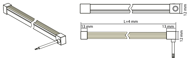
IP67 Glued Endcap - Left side outlet
