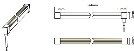
IP67 Glued Endcap - Bottom outlet
