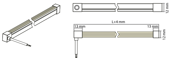
IP67 Glued Endcap - Right side outlet
