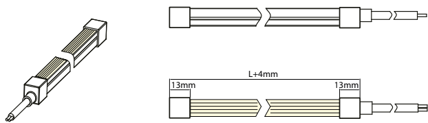
IP67 Glued Endcap - Axis outlet
