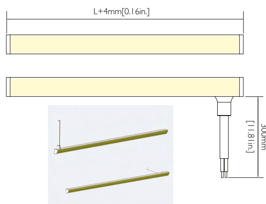
IP67 No dark Endcap - Left side outlet
