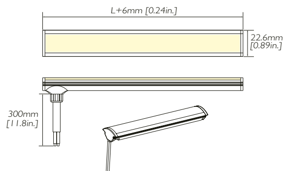
IP67 No dark Endcap - Bottom outlet
