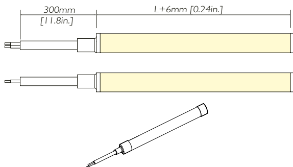
IP67 Glued Endcap - Axis outlet
