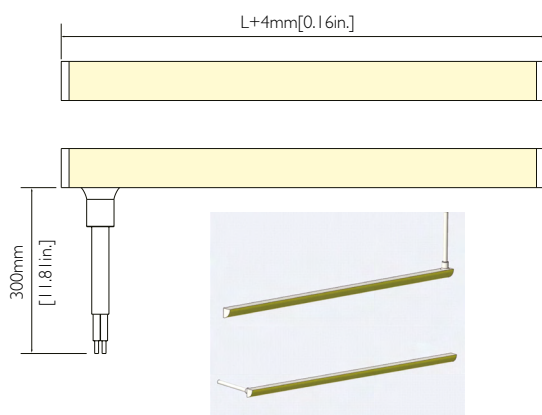
IP67 No dark Endcap - Right side outlet
