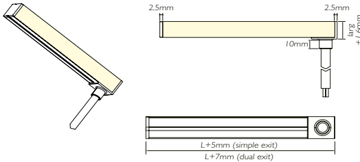
IP67 No dark Endcap - Left side outlet
