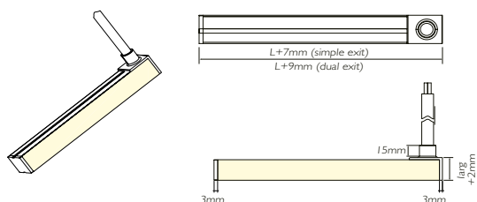
IP67 No dark Endcap - Right side outlet
