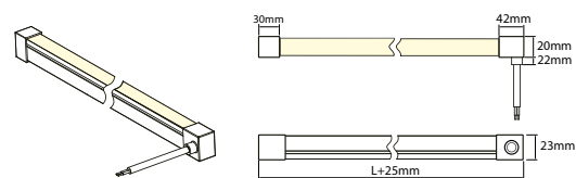
IP68 Dual injection-moulded Endcap - Left side outlet
